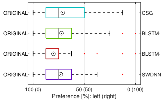
Fig. 7. Comparison of the CSG model and the baseline models with videos generated with the original lip motion sequences. The bars represent the first and third quartiles. The circle represents the mean values for each condition, the dash lines represent the minimum and maximum values, the vertical gray lines represent the medians, and the red dots represent outliers.
