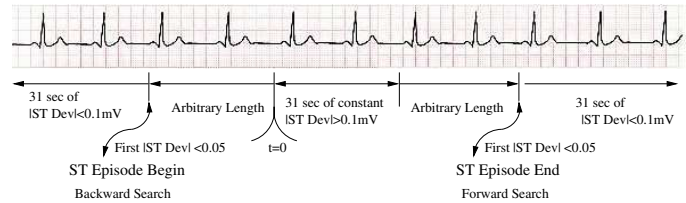
Figure 2. ST-Episode Detection
